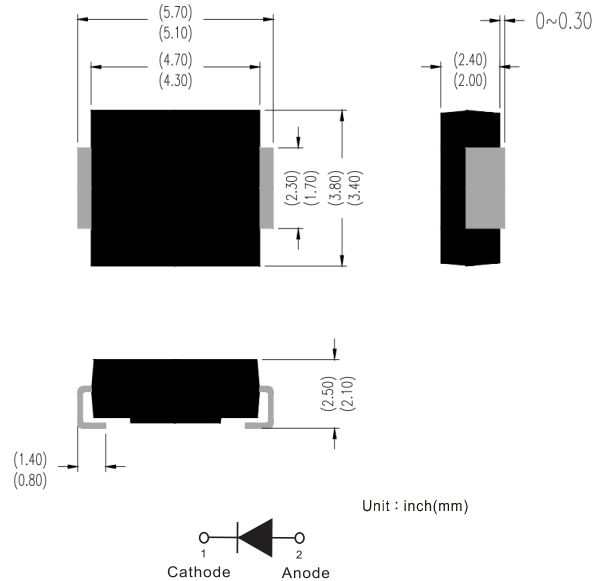
DO-214AA (SMB)
